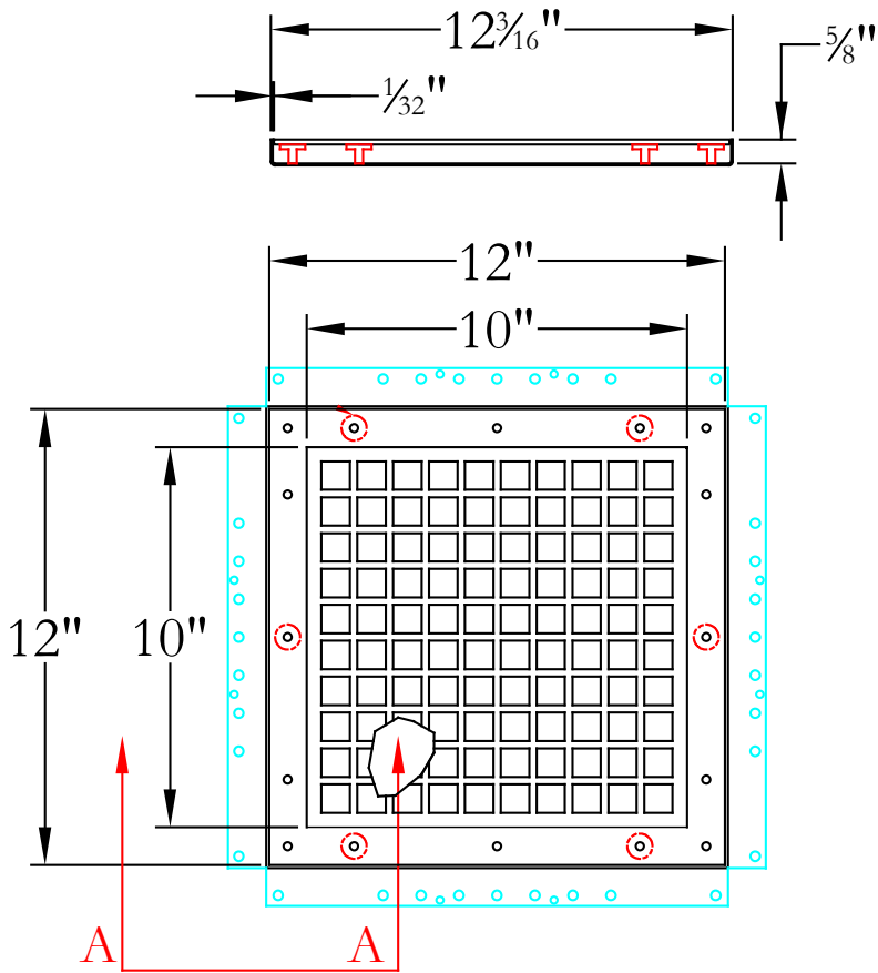
Square 10X10 Return w/ Flush Mount Can
